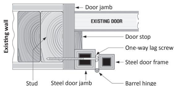
Inset mount
