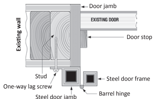
Surface mount w/tabs
