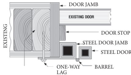
INSET MOUNT W/SURFACE
