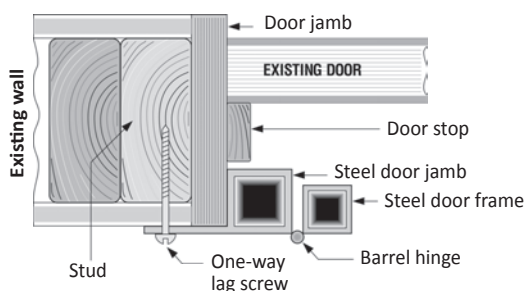
Inset mount w/surface tabs
