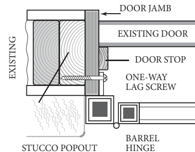
INSET MOUNT W/ TAB (SPECIAL TAB PLACEMENT)
