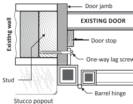
Inset mount w/ tab (Special tab placement)
