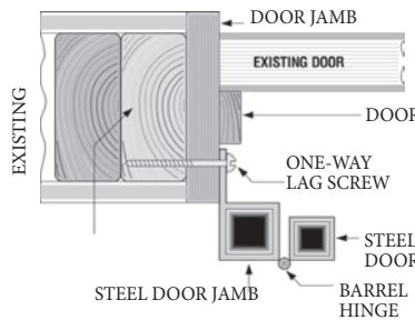
INSET MOUNT W/
