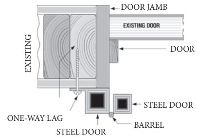
SURFACE MOUNT W/TABS
