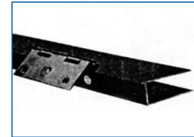
Extruded aluminum hinge side adjustment channel
