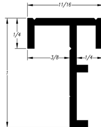
Security door "T" - astragal
